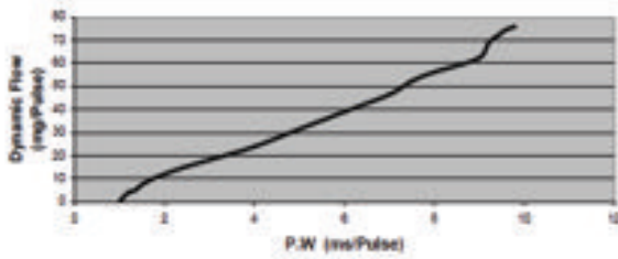
Characteristic Injector Flow
