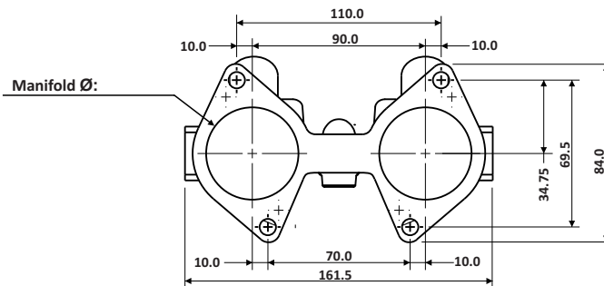
INTAKE MANIFOLD FLANGE FACE
