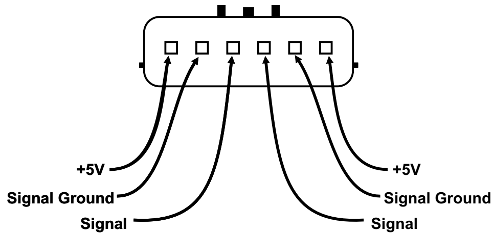
Connector - Male Pin View
